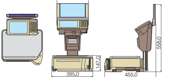
SM-5500EV EL (Elevated Elexy with 2nd printer)
