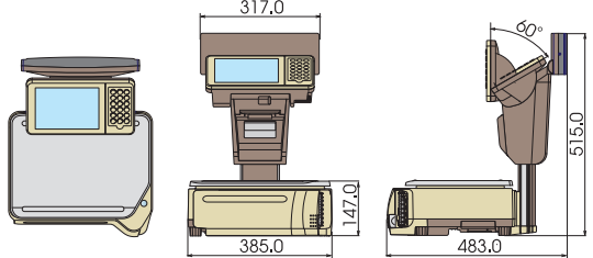
SM-5500EV EL (Elevated Elexy with 2nd printer)
