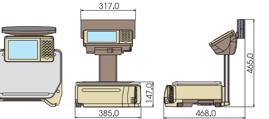
SM-5500EV (Elevated)
