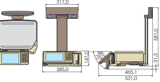
SM-5500EV (Elevated)
