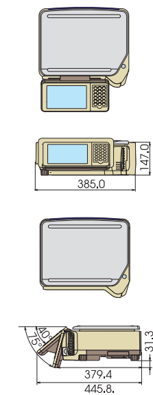
SM-5500B (Bench)
