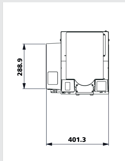
Cassette Labeller Technical Drawings Front
