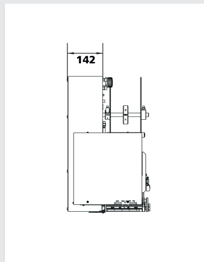
Signature Labeller Technical Drawings (Touch Applicator)
