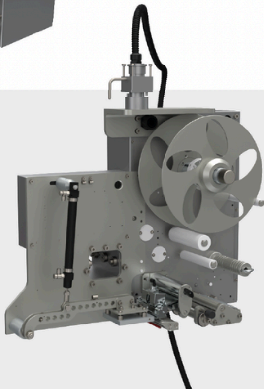
Front Applicator
